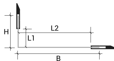
- H = L1 + 13 \text{ mm} - 1/2" B = L2 + 13 \text{ mm} - 1/2"
